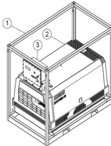
3D VIEW
